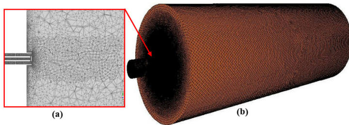
Figure 3. Computational domain grid: (a) Mesh refinement visualization near the coaxial burner exit, (b) Combustion chamber
