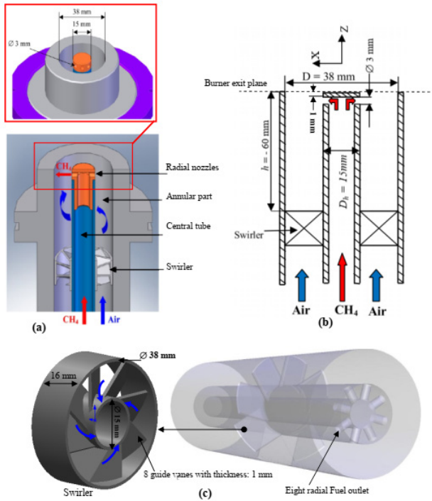
Figure 1. Coaxial swirl burner configuration [24, 25, 27] (a), 2D view of burner dimensions (b) and 3D view of the swirled burner (c)
