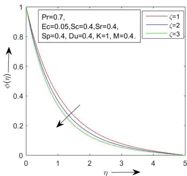
Figure 13. Concentration profile vs \zeta .
