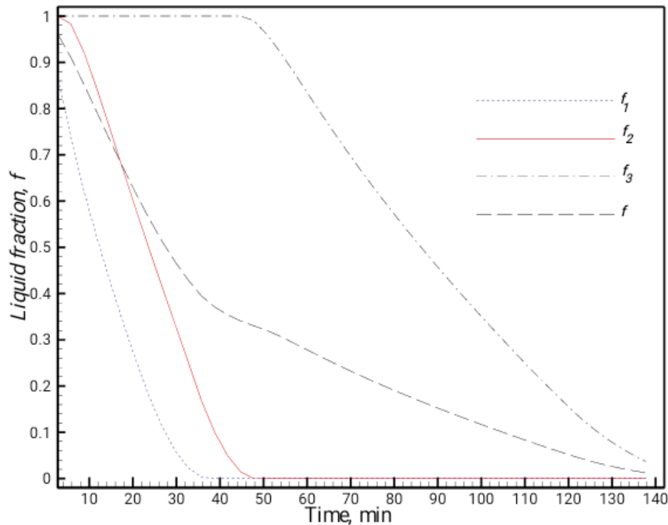
Figure 4. Time progression of the PCM liquid fraction.
