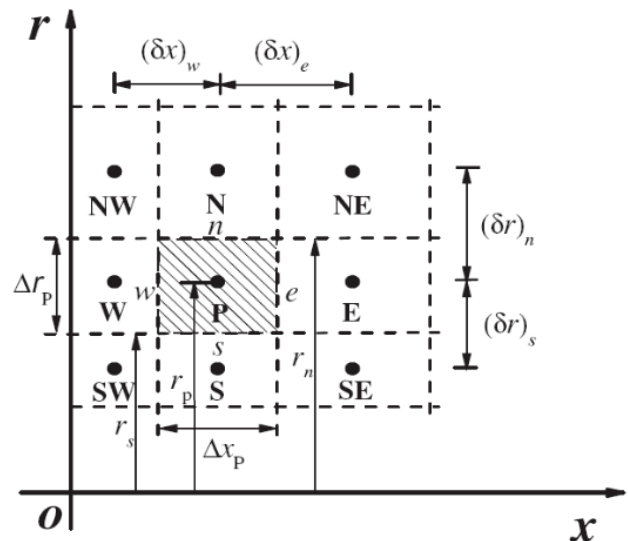
Figure 2. Control volume.
