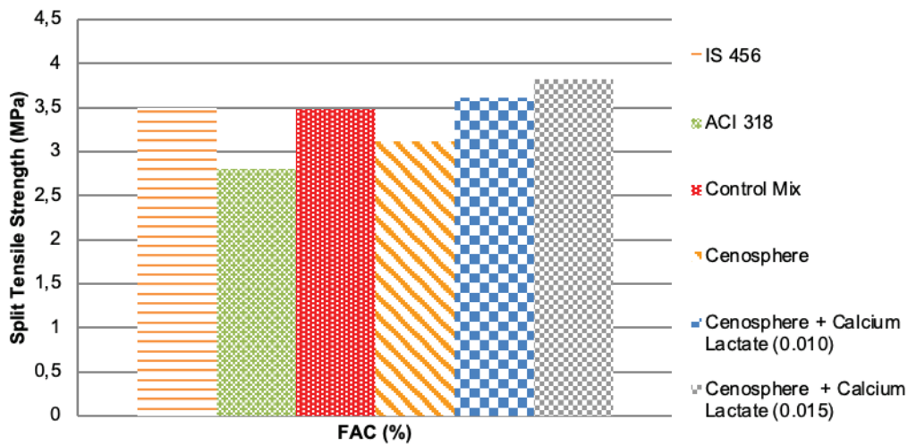
Figure 10. Split tensile strength (MPa) vs materials and codes for replacement of cement by cenosphere (10%).
