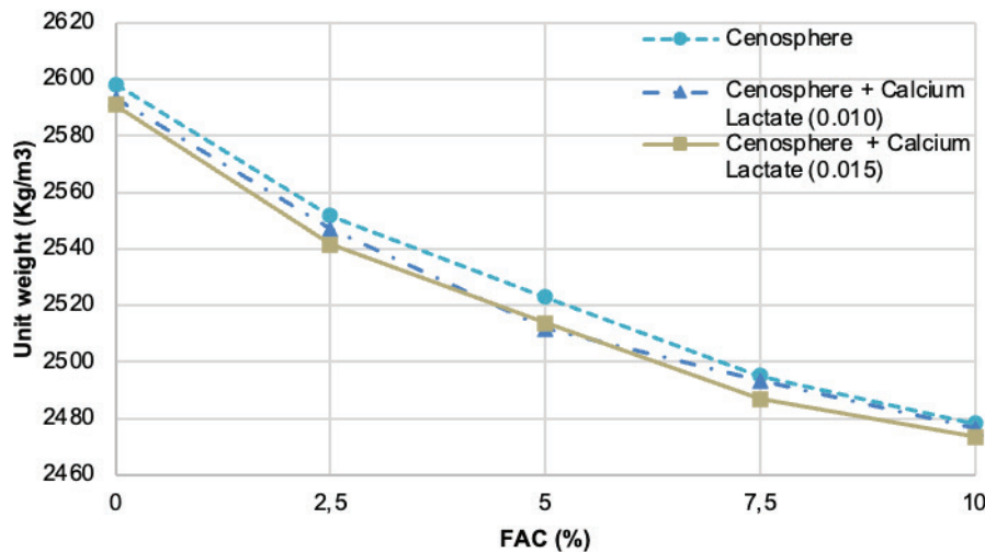
Figure 3. Unit weight (Kg/m 3 ) Vs FAC (%).
