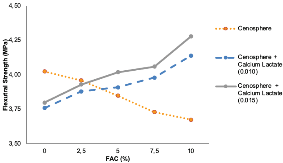
Figure 8. Flexural strength (MPa) Vs FAC (%).
