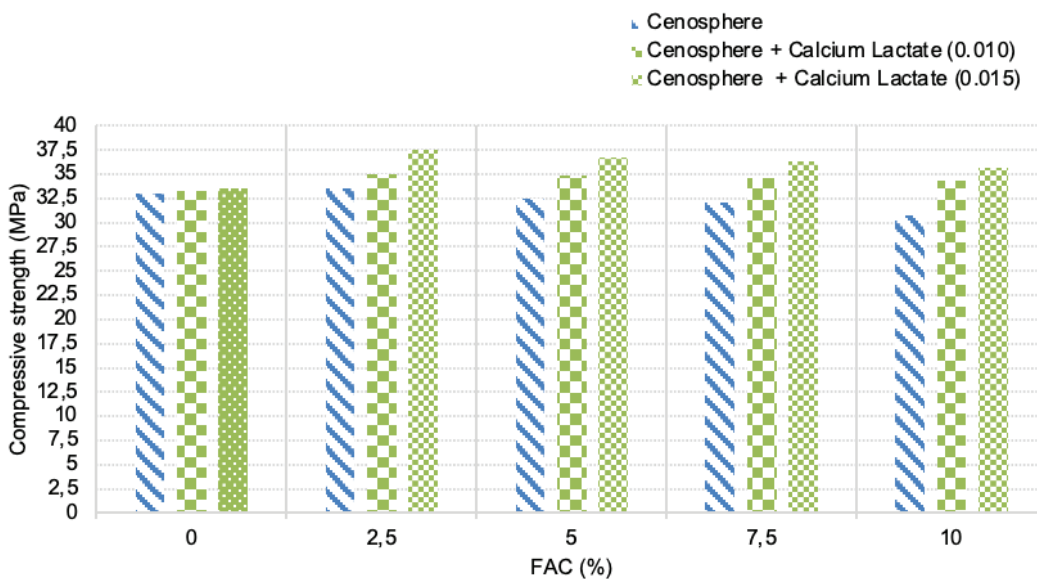
Figure 5. Compressive strength of concrete (Mpa) Vs FAC (%) at 28 days.
