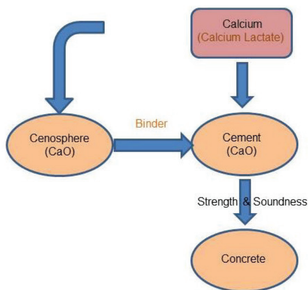
Figure 1. Flow diagram of cenosphere concrete mix.
