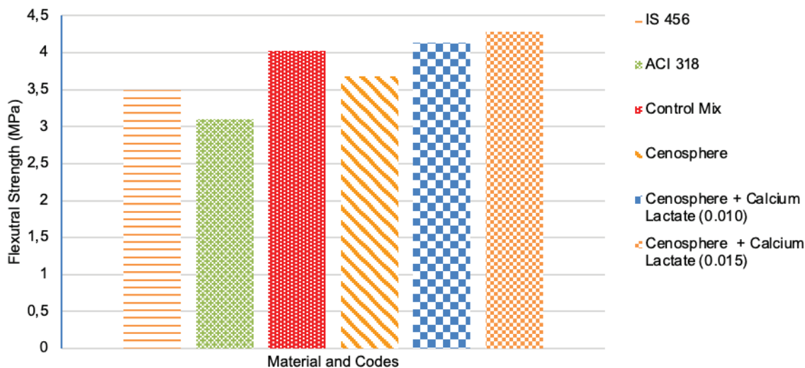
Figure 7. Flexutral strength (MPa) Vs Materials and Codes for replacement of cement by cenosphere (10%).
