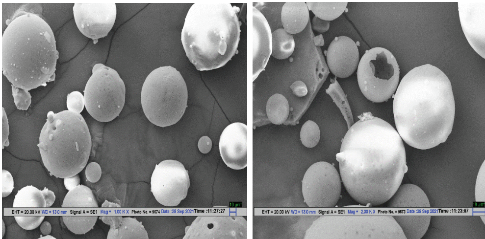
Figure 2. SEM image of cenosphere.
