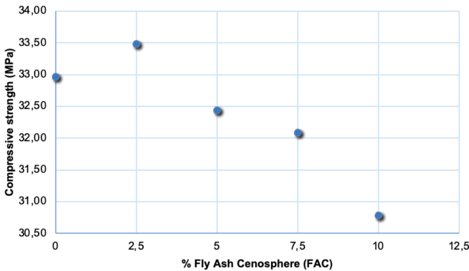
Figure 4. Compressive strength of FAC concrete at 28 days.
