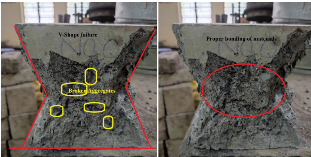
Figure 6. Failure pattern of compression member.
