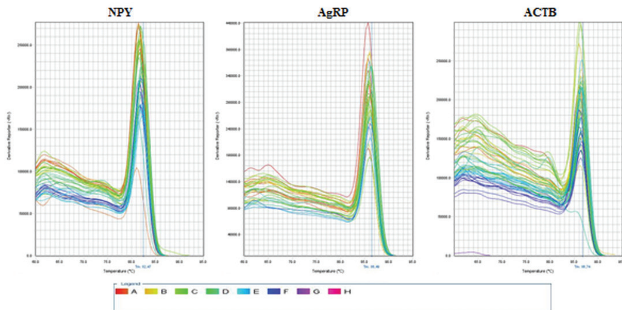
Figure 1. Melting curve image of the Real-Time PCR reaction of the experimental groups. A/B/C/D/E/F/G/H represent samples in each row on the plate.
