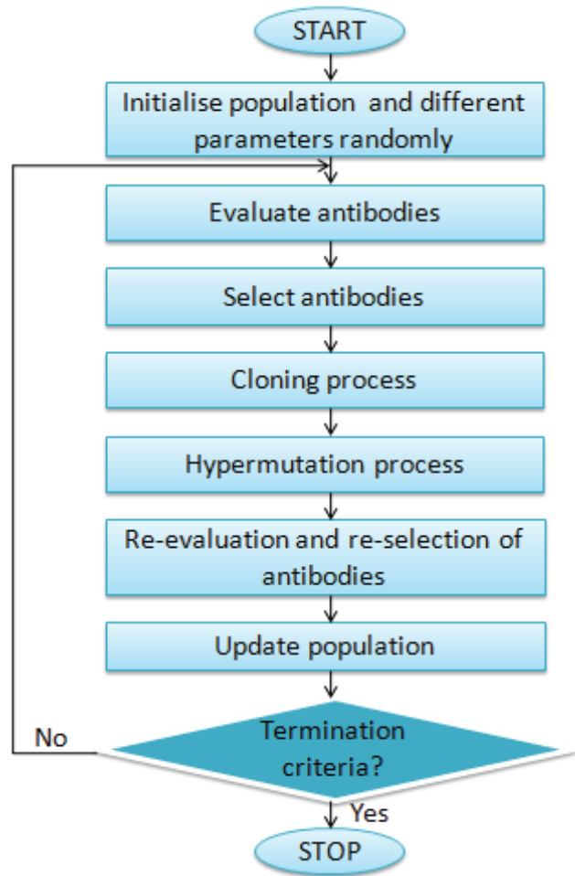
Figure 6. Clonal selection algorithm [28].
