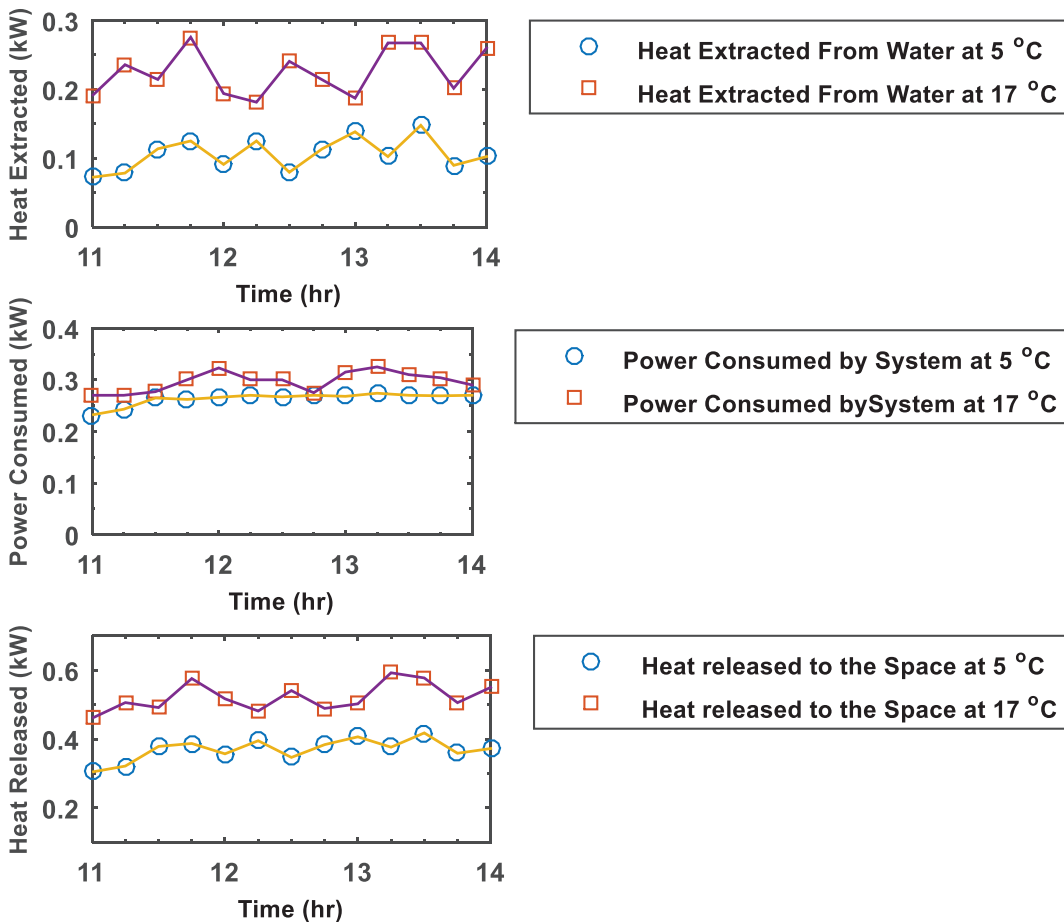
Figure 4. Effect of water source temperature on different energy flow rates.
