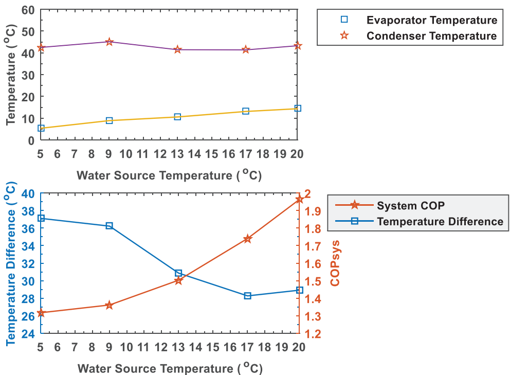
Figure 10. Effect off temperature difference between the condenser and evaporator on system performance.
