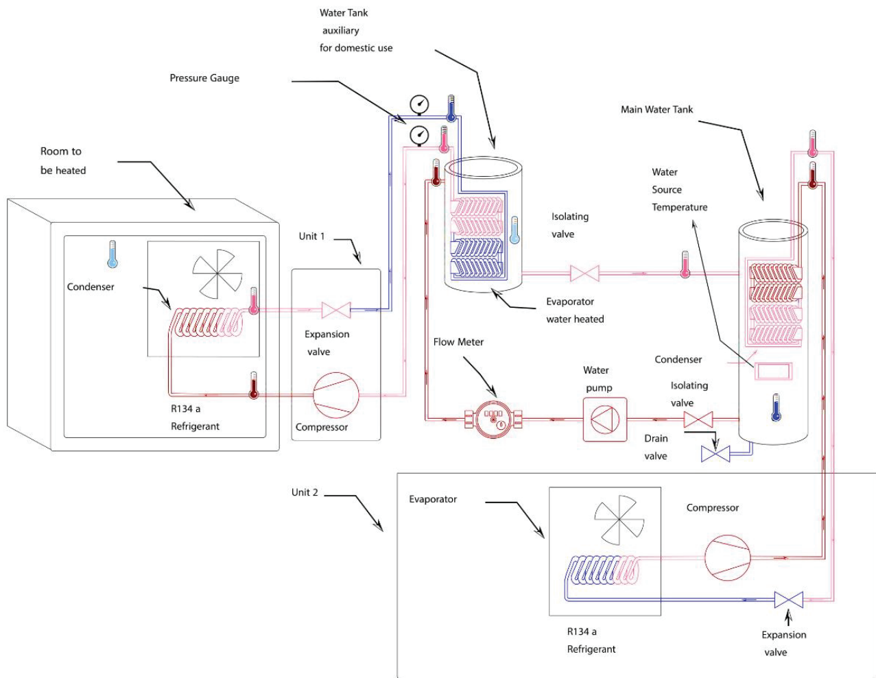
Figure 1. Schematic Diagram of the WSHP system in heating mode.
