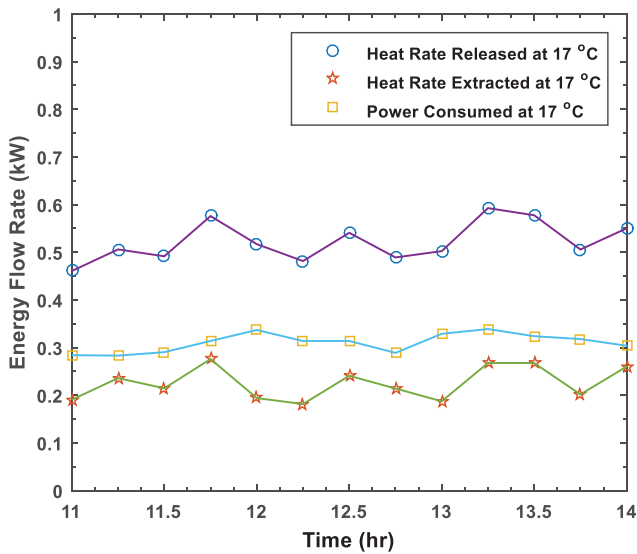
Figure 3. Changes of energy flow rates with time.
