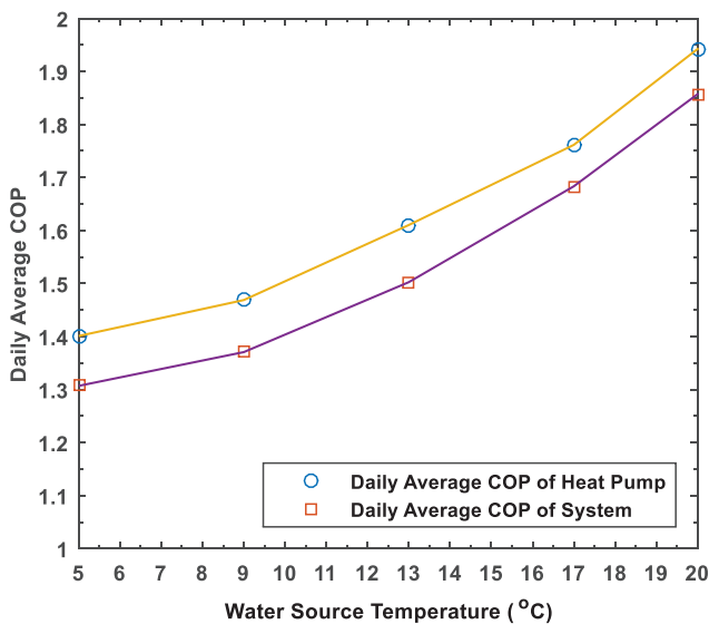
Figure 7. Effect of water source temperature on the daily average coefficient of performance.
