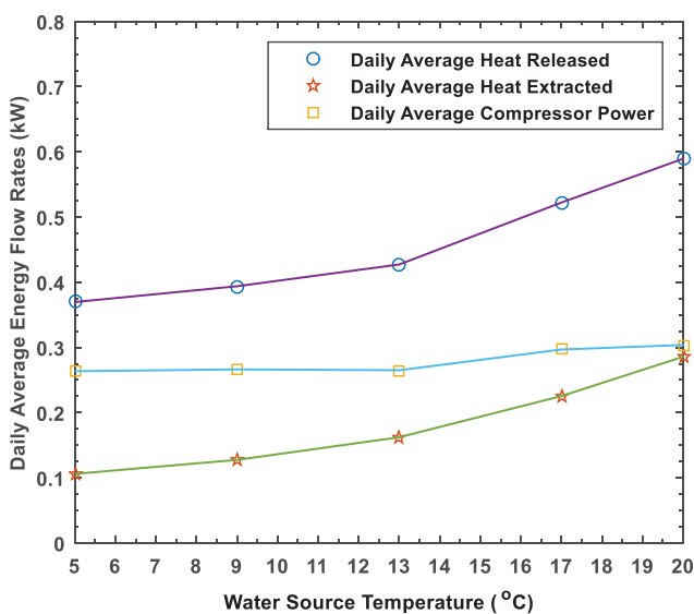
Figure 5. Effect of water source temperature on the daily average energy flow rates.
