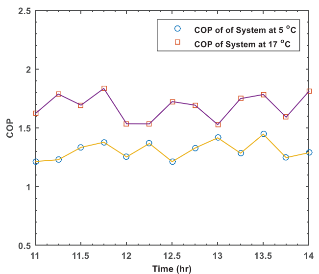
Figure 6. Effect of water source temperature on the coefficient of performance.
