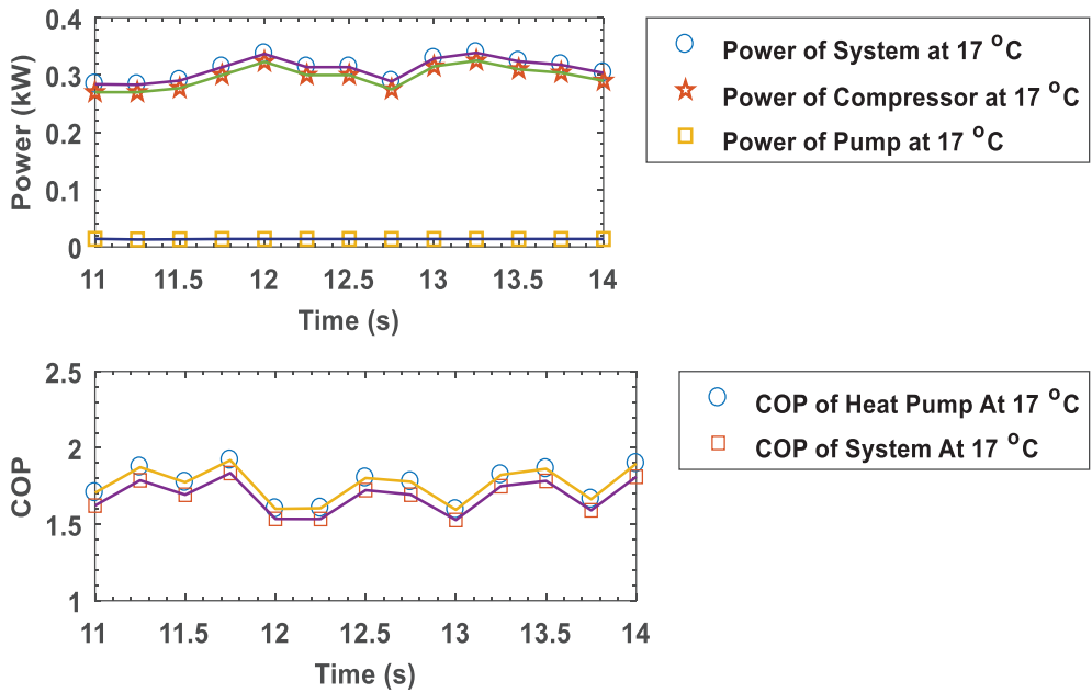
Figure 9. Effect of pumping energy on the coefficient of performance.
