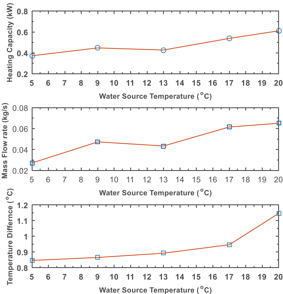
Figure 11. Effect of heating capacity on temperature difference and the flow rate of water loop.
