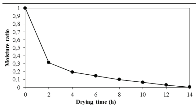
Figure 6. Hawthorn MR curve (drying time: 14 hours).
