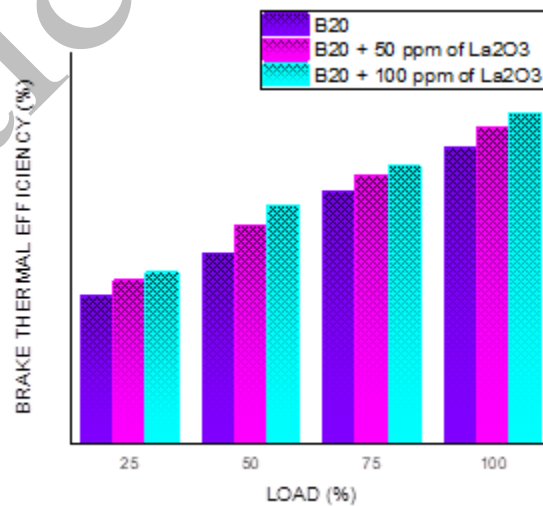
Figure.6 Variation of brake thermal efficiency with load
