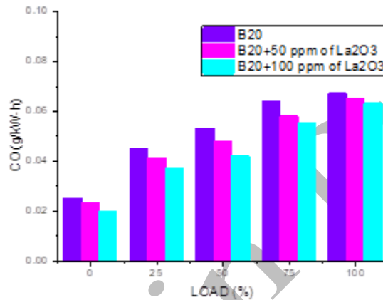
Figure.7 Variation of carbon monoxide with load
