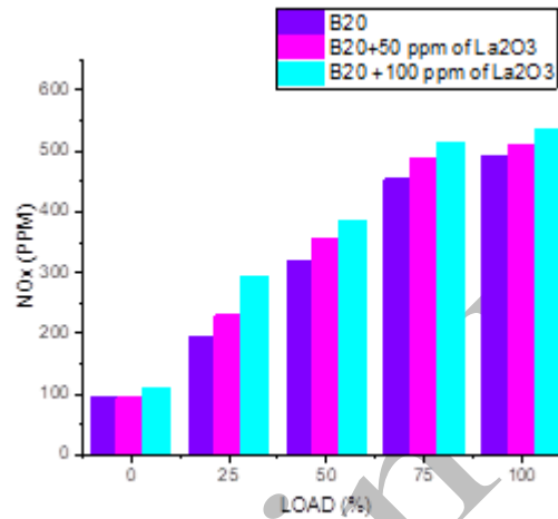
Figure.9 Variation of nitrogen oxide with load
