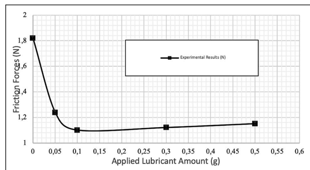
Figure 7. Oil amount-friction force relationship.
