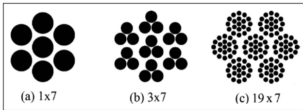
Figure 2. Inner cable winding forms used in the control cables [7].
