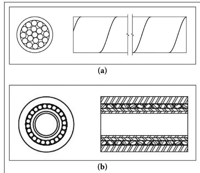
Figure 3. Sketch of inner cable and conduit; (a) 1x19 coiled armoured inner cable (b) PTFE coated, steel braided and PVC coated conduit.
