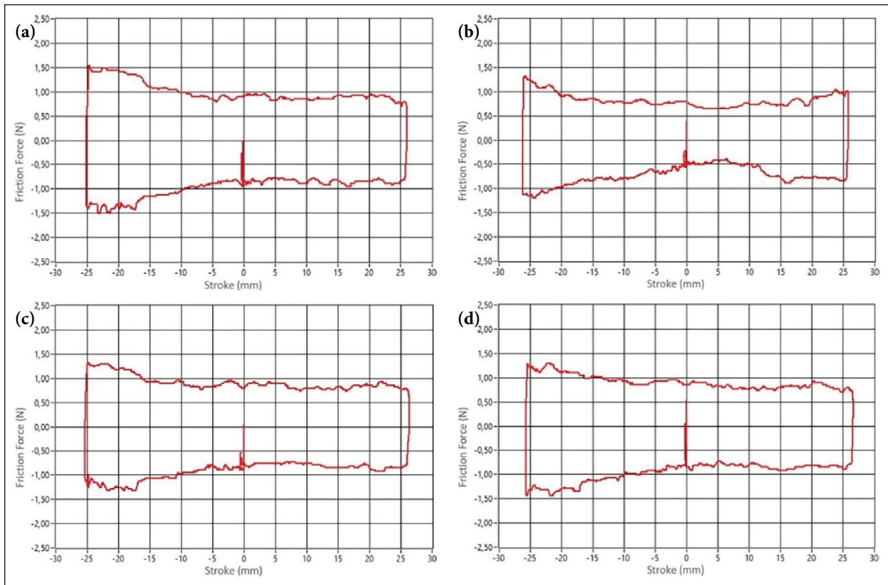
Figure 6. Results of friction tests under lubricated condition; (a) 0.05 g lubricant, (b) 0.1 g lubricant, (c) 0.3 g lubricant, (d) 0.5 g lubricant.
