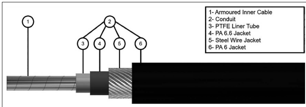
Figure 1. Elements of control cable.
