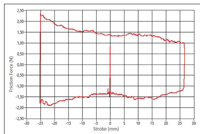
Figure 5. Results of friction tests of dry control cable.
