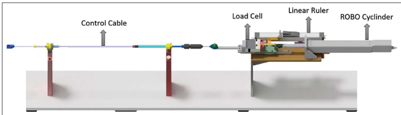
Figure 4. The experimental setup.
