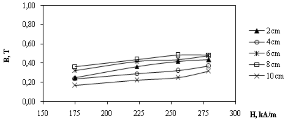
Figure 8. The average magnetizing curve of the magnetized bed (d=12 mm)
