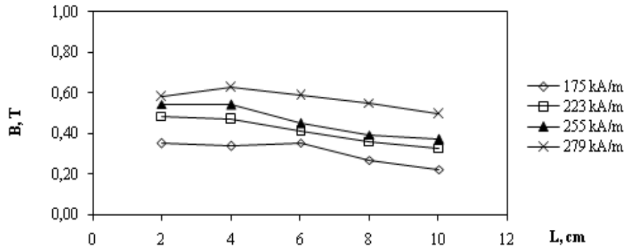
Figure 5. The magnetic induction field profiles of the magnetized bed (d=6 mm)
