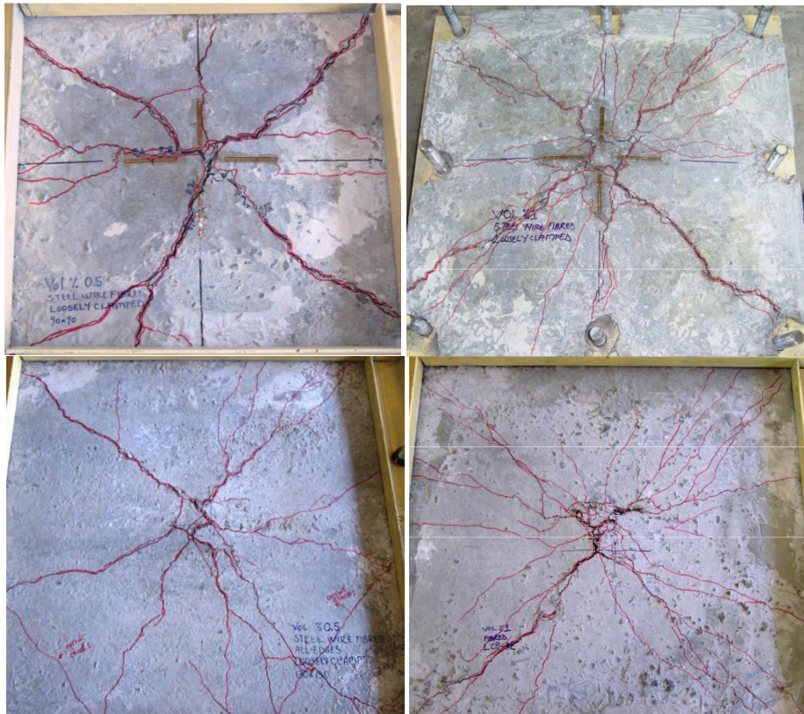
Figure 12. Fracture mechanisms of the high strength fiber concrete test slabs[18]
