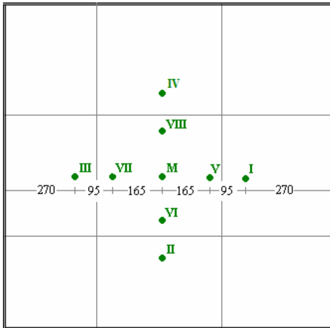
Figure 5. Deflection measurement points for 1060x1060 mm free-span slabs
