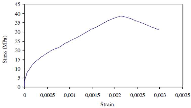
Figure 11. Stress-strain curve for ordinary (1.0% fiber) concrete
