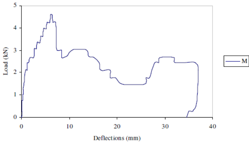
Figure 18. Load-deflection behavior of AGL4
