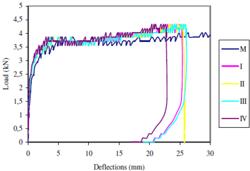
Figure 21. Load-deflection behavior of AGLB4I
