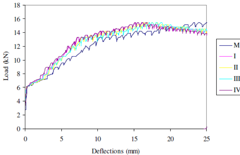
Figure 16. Load-deflection behavior of AL4I
