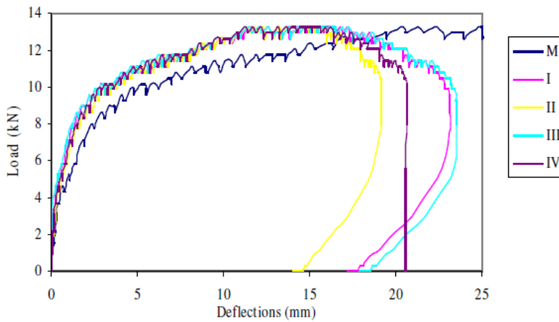
Figure 17. Load-deflection behavior of ALB4I
