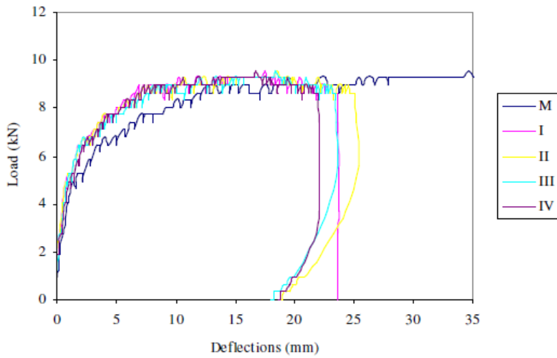
Figure 15. Load-deflection behavior of ALB4
