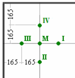
Figure 4. Deflection measurement points for 660x660 mm free-span slabs
