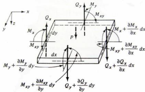
Figure 1. Internal forces generated within a plate [1,2]
