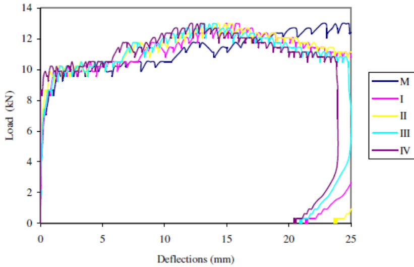
Figure 14. Load-deflection behavior of AL4
