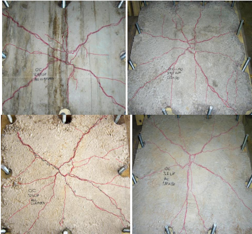
Figure 13. Fracture mechanisms of the ordinary fiber concrete test slabs[18]
