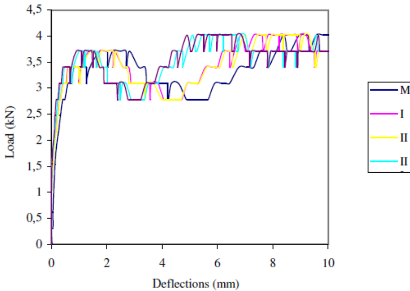
Figure 20. Load-deflection behavior of AGL4I
