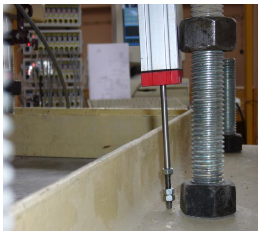
Figure 7. Support rotation measurements
