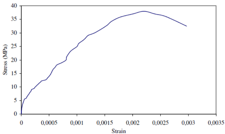
Figure 10. Stress-strain curve for ordinary (0.50% fiber) concrete
