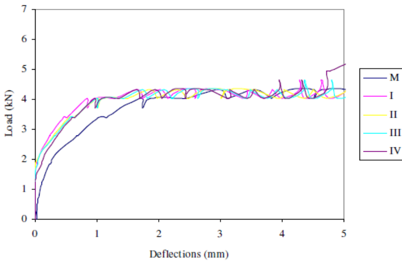
Figure 19. Load-deflection behavior of AGLB4
