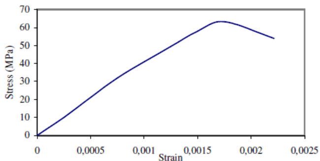
Figure 9. Stress-strain curve for high-strength (1.0% fiber) concrete
