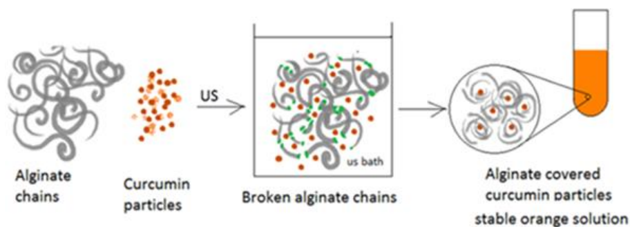
Figure 2. Schematic representation of curcumin solubilization by alginate in ultrasound medium.
